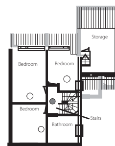
Recommended placing for the Smoke Alarm: 1 smoke detector on each floor.
