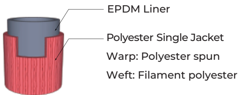
Single Jacket Hose
