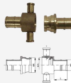
BS336 Coupling in Brass & Aluminum
