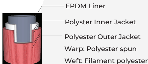
Double Jacket Hose
